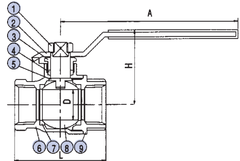
DIMENSIONS - 2032T
